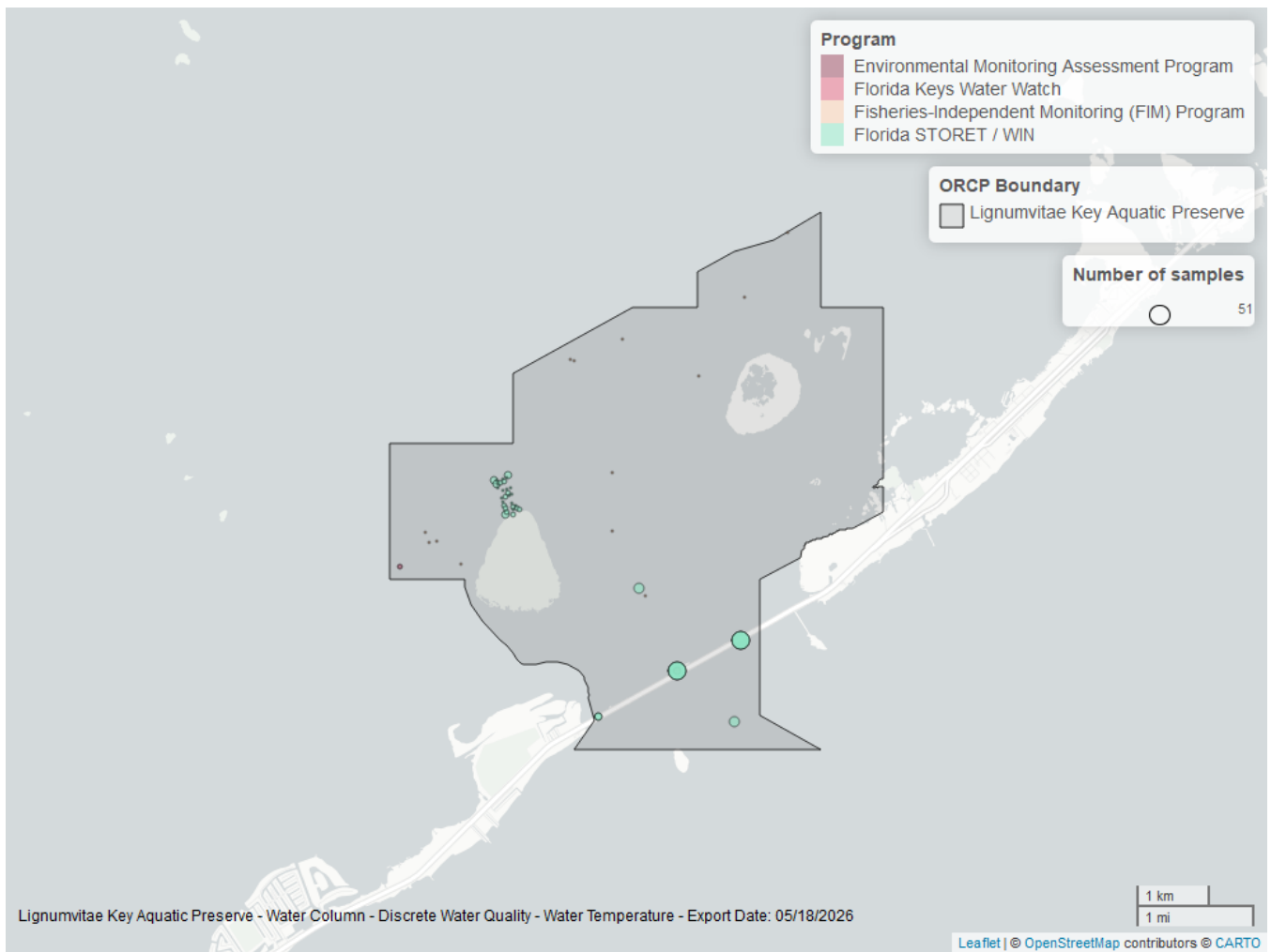
Figure 16: Map showing location of discrete water quality sampling locations within the boundaries of Lignumvitae Key Aquatic Preserve . The bubble size on the maps above reflect the amount of data available at each sampling site.
